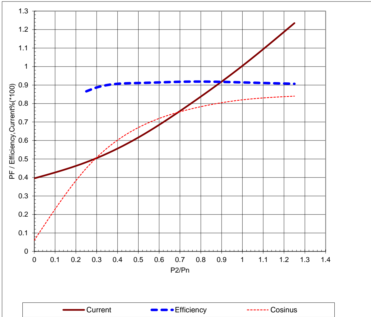
Load characteristics (IEC 60034-2-1:2014) Data based on situation 01/06/2017
